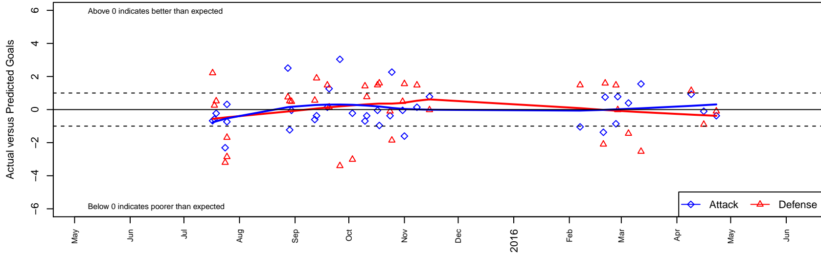
FC Portland Navy B03 Dots are actual minus expected GF (blue circles) and GA (red triangles). Blue line is smoothed change in attack strength. Red is smoothed change in defense strength.
